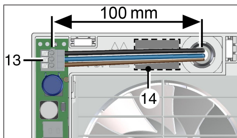
13 Spring clip
