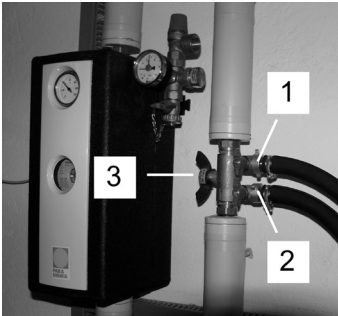
3. Connect pressure hose (1) and return hose (2) to the fill/vent valves and open valves. Close stop valve (3).
