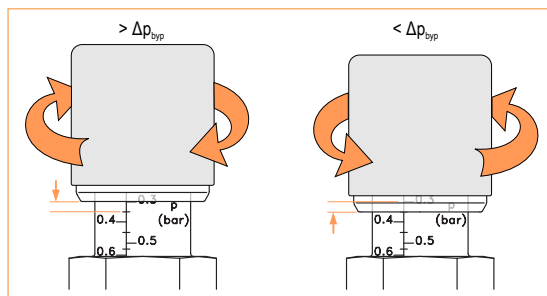
(b) Adjustment of by-pass differential pressure, \Delta p_{byp} .
