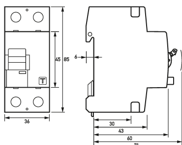
Dimensioned drawing residual current circuit-breaker DFS 2 016-2/0,30-A
